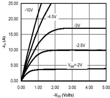
Fig 1: On-Region Characteristics
