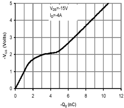
Figure 7: Gate-Charge Characteristics
